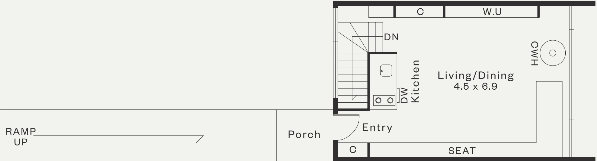
GROUND FLOOR
