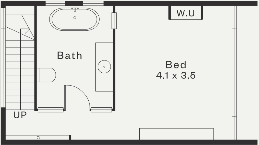
LOWER FLOOR
